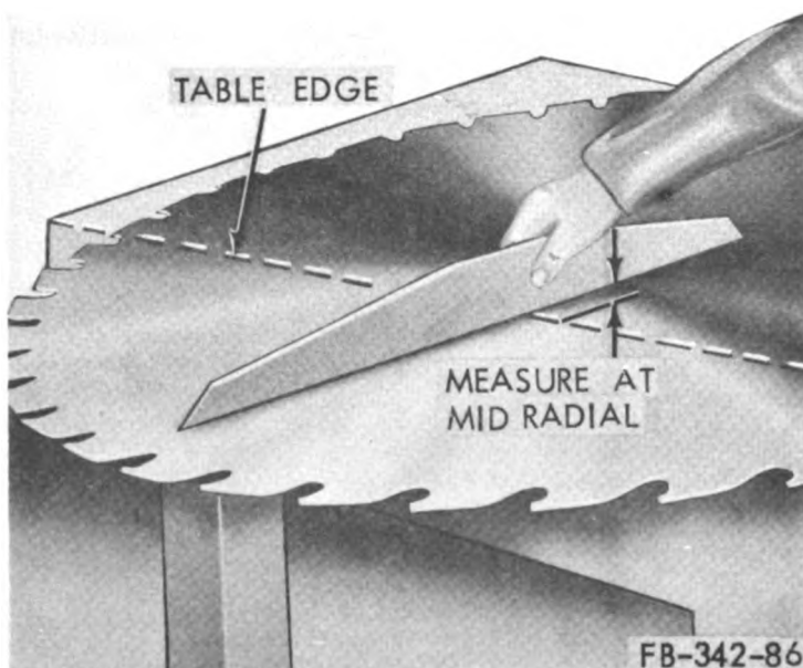
Figure 10-3. Method of measuring tension in a circular saw.
